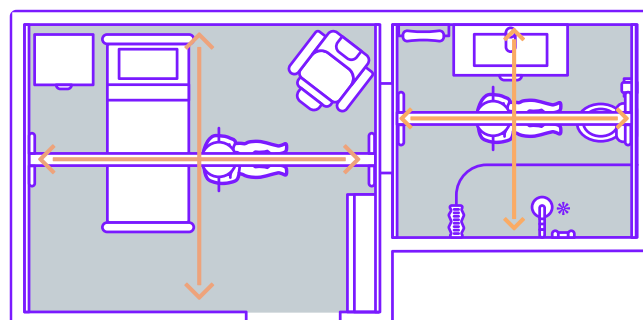
XY systems with door connector
